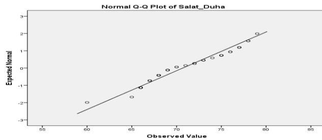
Grafik IV.1 Normal Q-Q plot salad Duha
