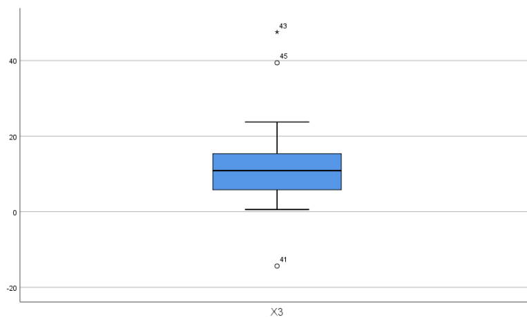
Boxplot X3
