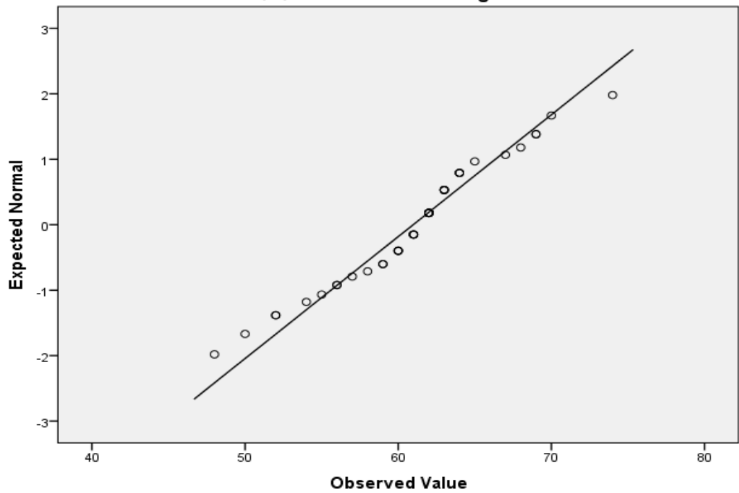
Normal Q-Q Plot of Komitmen Organisasi
