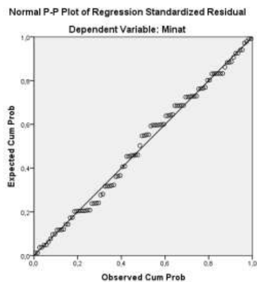
Gambar 4.1 Hasil Uji Normal P-Plot
