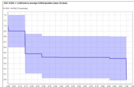
Figure 3. Result of AUC (Area Under the ROC Curve) at C4.5 (79 records)
