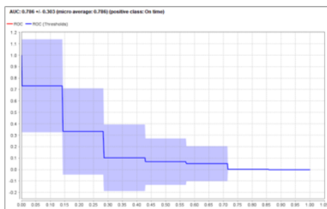
Figure 5. Result of AUC (Area Under the ROC Curve) at Naïve Bayes (79 records)
