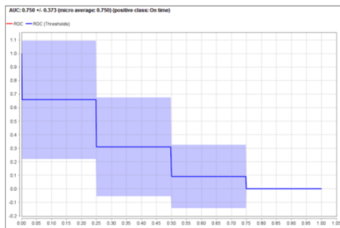
Figure 10. Result of AUC (Area Under the ROC Curve) at Naïve Bayes (50 records)
