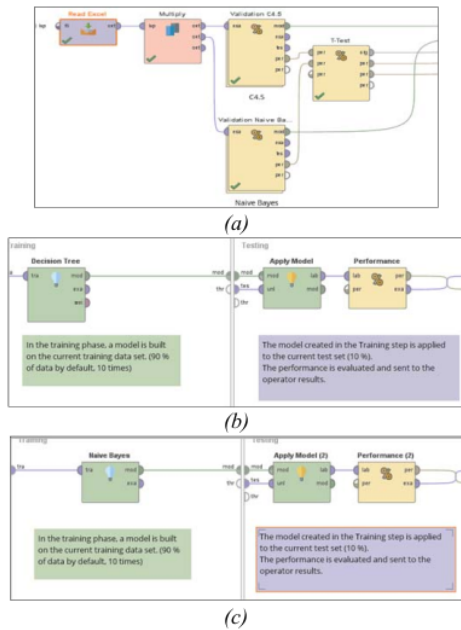
Figure 1. Classification Method Comparison Design Model (a)(b)(c)
