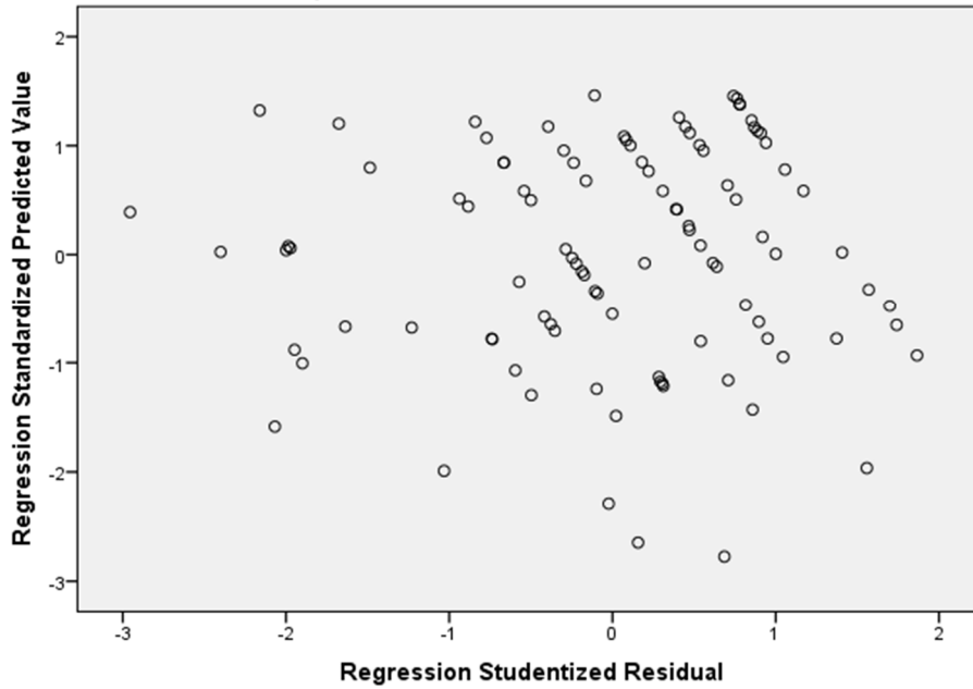
Scatterplot
