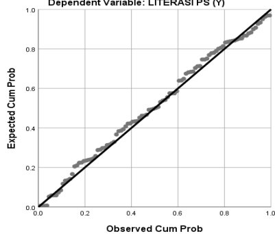
Normal P-P Plot of Regression Standardized Residual Dependent Variable: LITERASI PS (Y)
