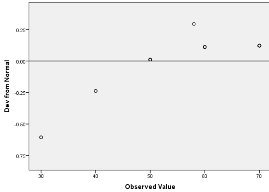
Detrended Normal Q-Q Plot of Hasi Pretest for Kelas= IPA2
