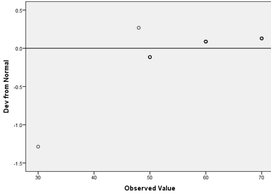
Detrended Normal Q-Q Plot of Hasi Pretest for Kelas= IPA1
