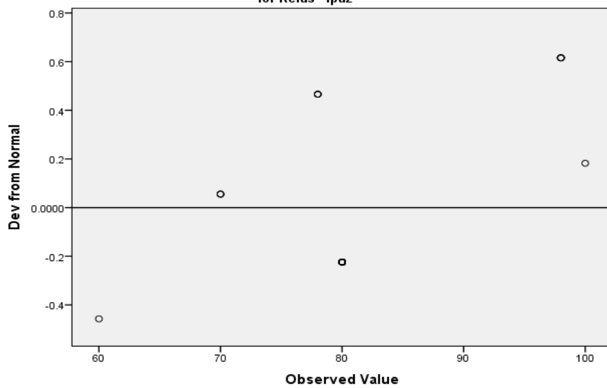
Detrended Normal Q-Q Plot of Hasil Postest for Kelas= Ipa2
