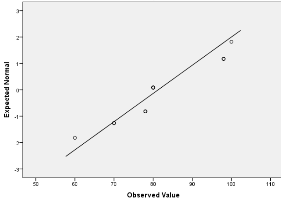
Normal Q-Q Plot of Hasil Postest for Kelas= Ipa2
