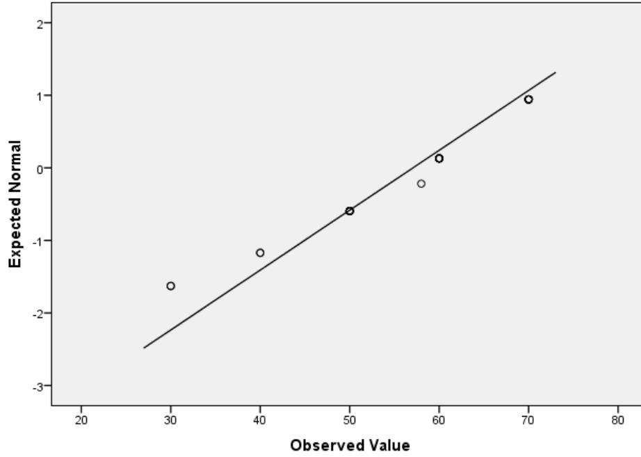
Normal Q-Q Plot of Hasi Pretest for Kelas= IPA2
