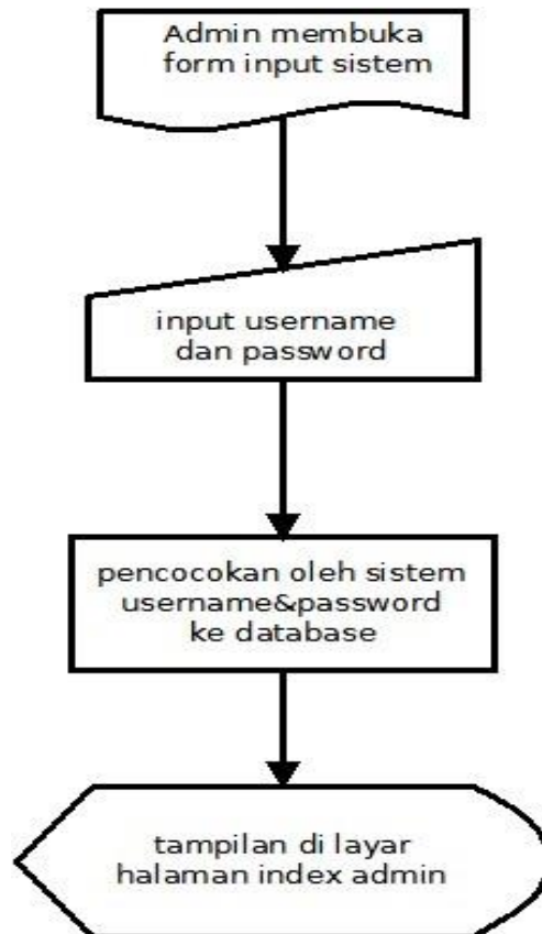
Gambar 4.18 Flowchart Transaksi
