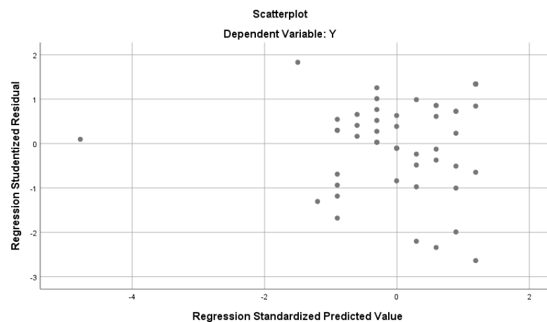
Gambar 4.1 Scatterplot
