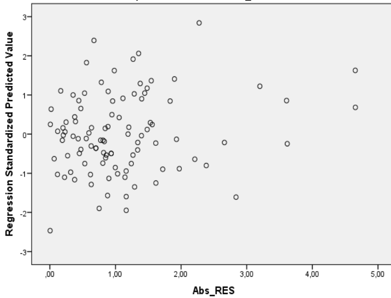
Scatterplot
