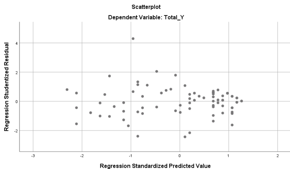
Gambar 4. 1. Scatterplot
