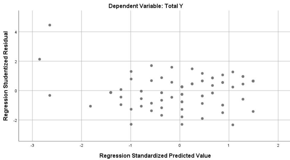
Scatterplot
